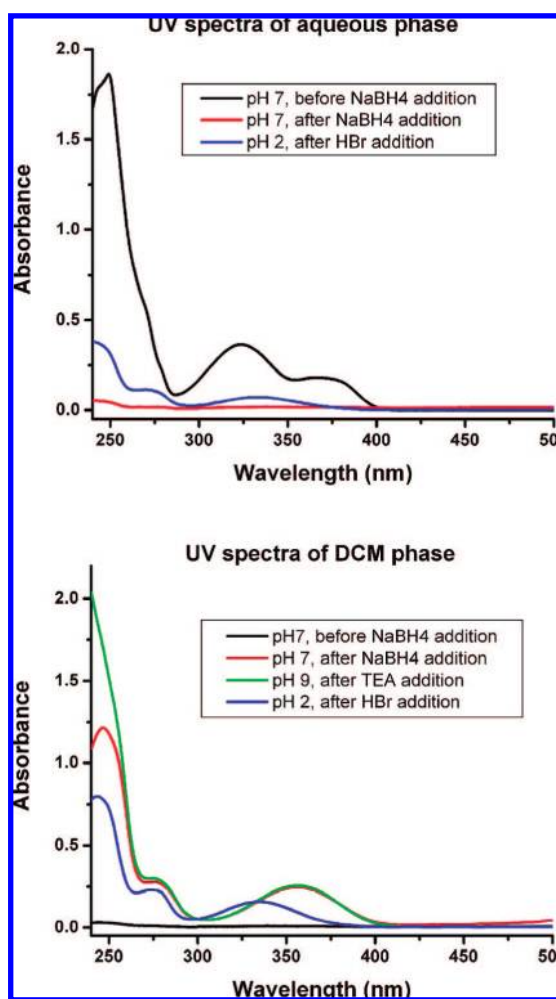
Figure 6. UV spectra of aqueous (top) and DCM (bottom) phases during reduction of AEP 3 to AEDP 4 under biphasic conditions: (i) before \text{NaBH}_4 addition, black curve; (ii) after \text{NaBH}_4 addition, red curve; (iii) after TEA addition, green curve; (iv) after excess HBr addition, blue curve.
