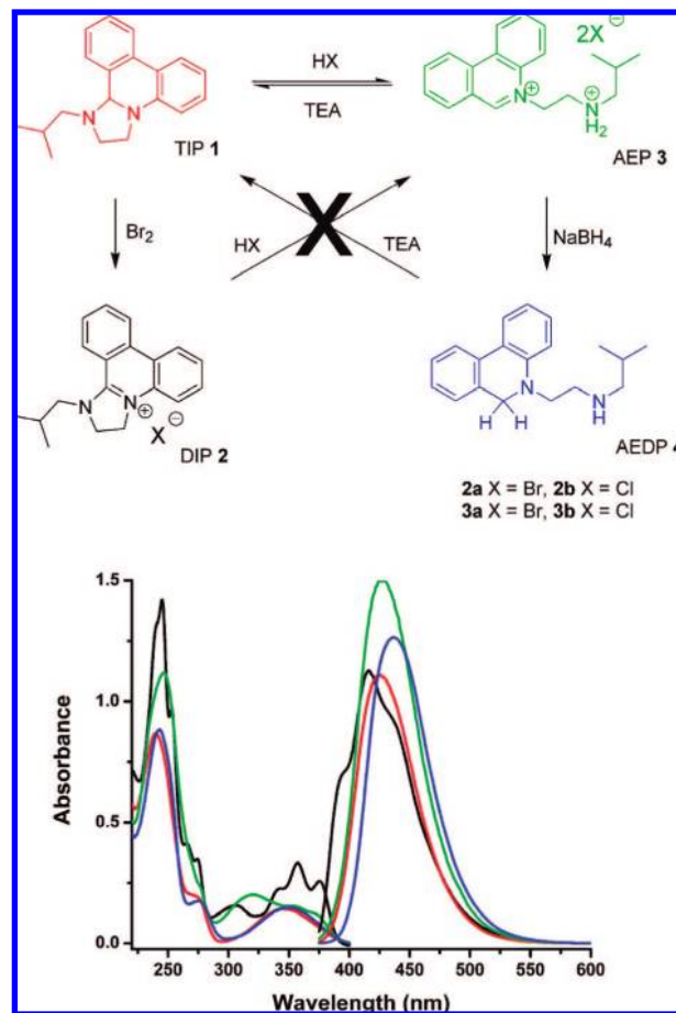
Figure 1. Reaction scheme and absorption (left) and emission (right) spectra for each of the four switchable states: (i) TIP, red curve; (ii) DIP, black curve; (iii) AEP, green curve; (iv) AEDP, blue curve. For absorption spectra, concentrations were 4 \times 10^{-5} M in acetonitrile. See Supporting Information for emission spectra conditions.
